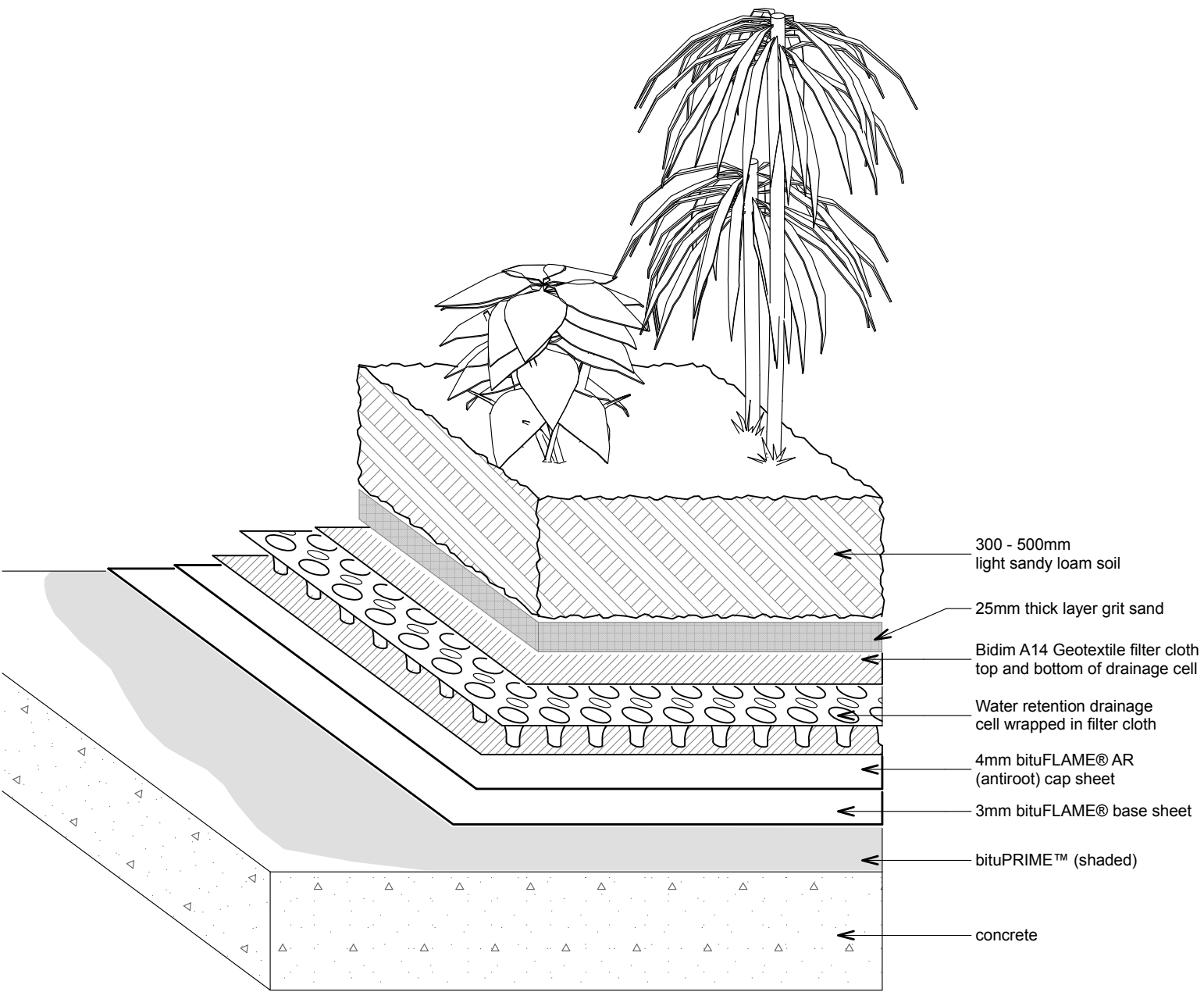
Green Roof bituFLAME (bF-AR) 3D CUTAWAY
