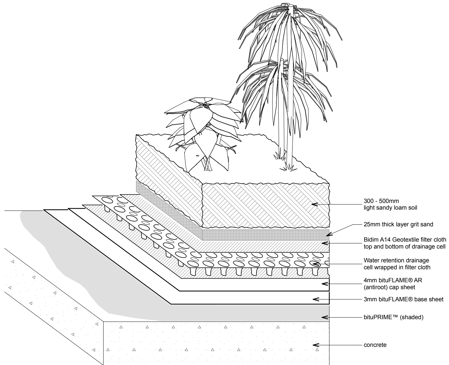
ecoROOF™ bituFLAME (bF-AR) 3D CUTAWAY
