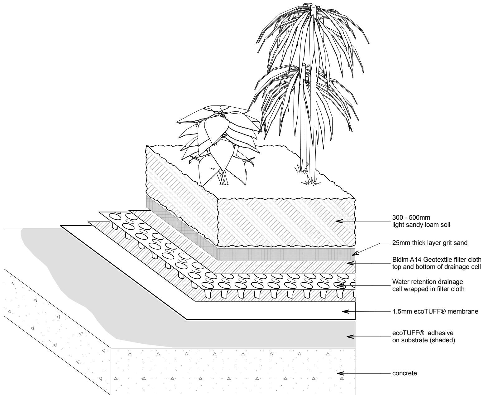
ecoROOF™ (TPO) 3D CUTAWAY
